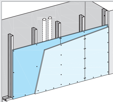
FR (2 x 25) W628 F(90)
