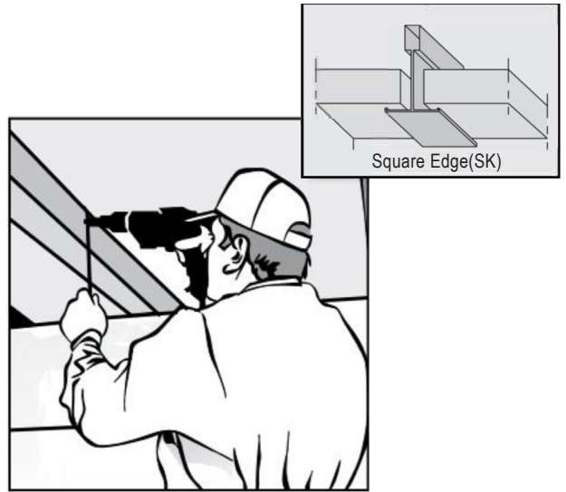
2. Fixing the hangers to the main soffit
